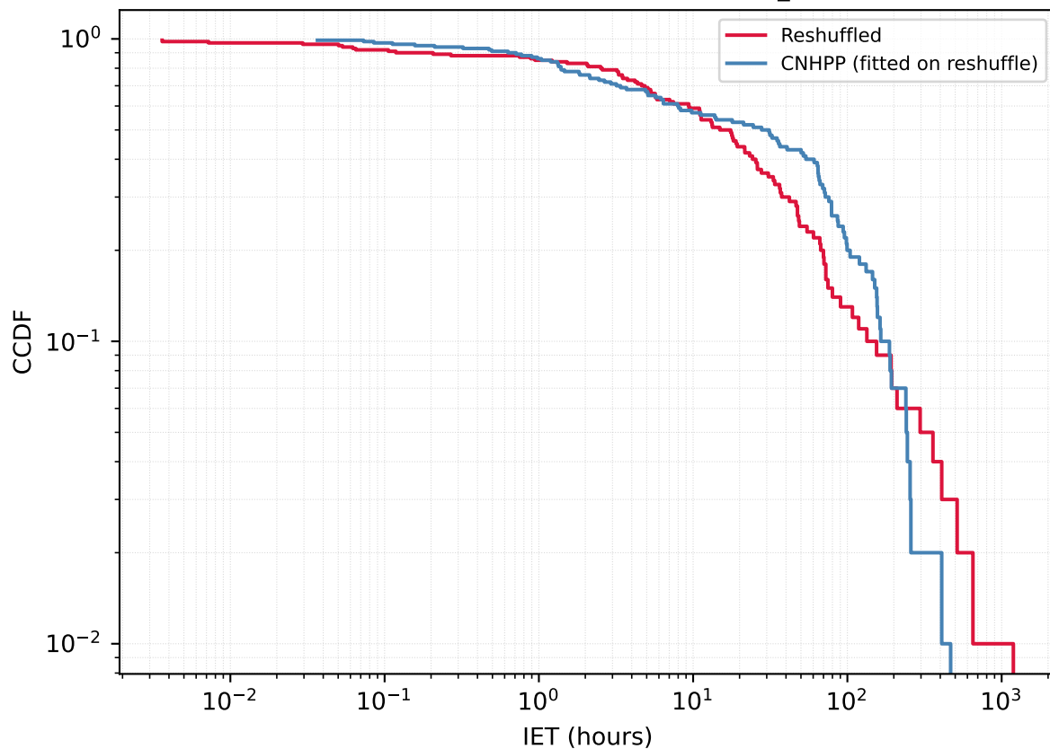
User 5992929865 - Reshuffled vs CNHPP A_{\text{fit}}=0.7992
